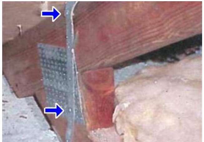
Roof to Wall Connection - Straps
